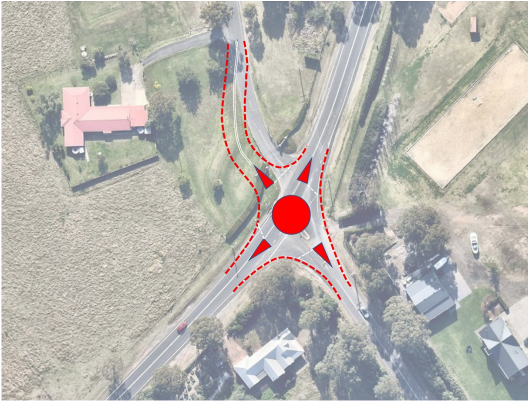
Figure 4.3: Roundabout Access
